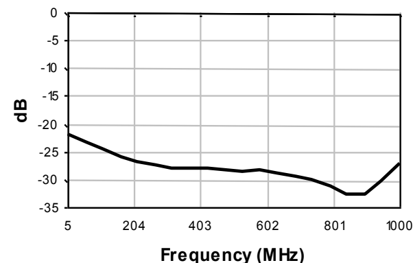
Return Loss: Coupled (Pin 4)
