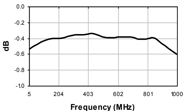
Main Line Loss (Pin6 - Pin1)
