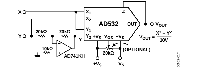
Figure 19. Differential of Squares Connection
