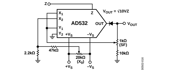
Figure 18. Square Rooter Connection
