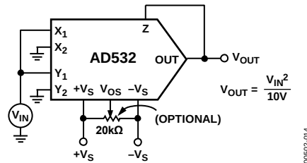
Figure 16. Squarer Connection
