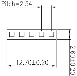
HOUSING
