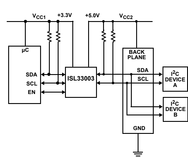
FIGURE 1. TYPICAL OPERATING CIRCUIT
