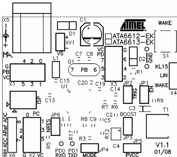
Figure 7-2. ATA6612/ATA6613 Board Component Placement; Top Side, Top View
