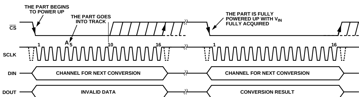
Figure 28. Exiting Power-Down Mode
