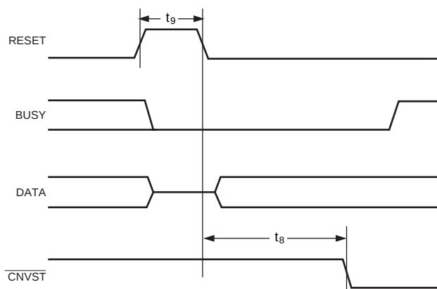
Figure 12. RESET Timing
