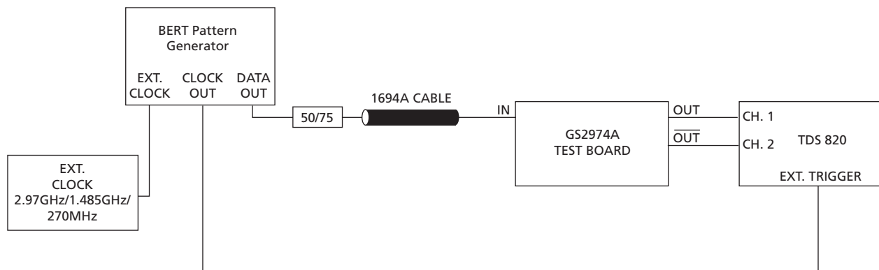
Figure 2-1: Test Circuit
