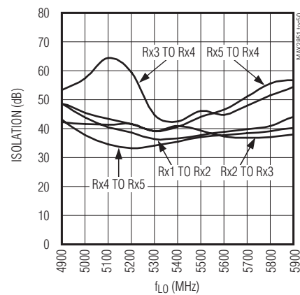
Rx CHANNEL ISOLATION
