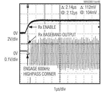
POWER-ON DC OFFSET CANCELLATION WITH INPUT SIGNAL
