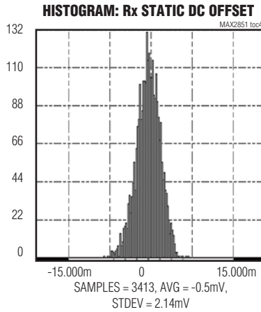
POWER-ON DC OFFSET CANCELLATION WITHOUT INPUT SIGNAL
