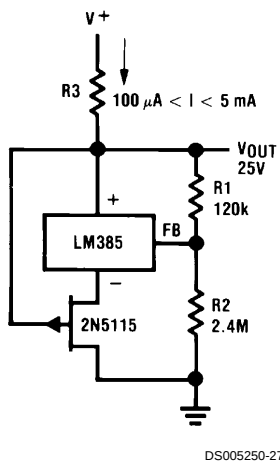
25V Low Current Shunt Regulator
