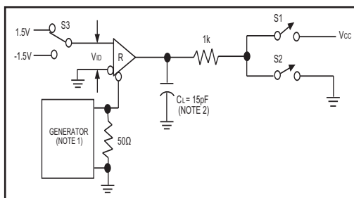
Figure 7. Receiver Enable and Disable Timing Circuit
