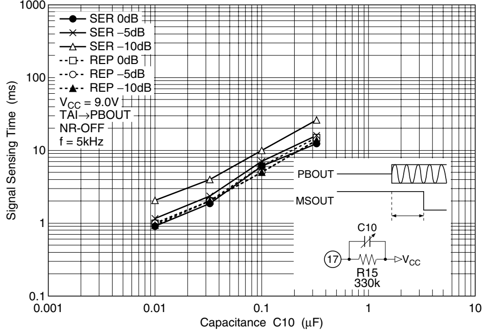
Signal Sensing Time vs. Capacitance (HA12216F)
