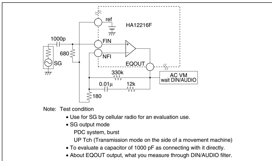
Figure 7 Test Circuit
