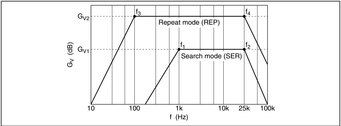
Figure 5 Frequency Response
