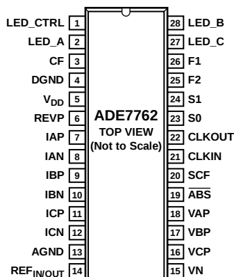
Figure 4. Pin Configuration
