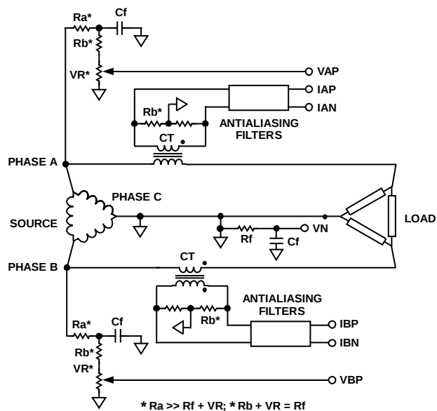
Figure 22. 3-Phase 3-Wire Meter Connection with ADE7762
