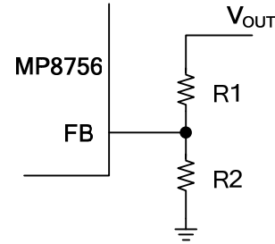
Figure 7: Feedback Network
