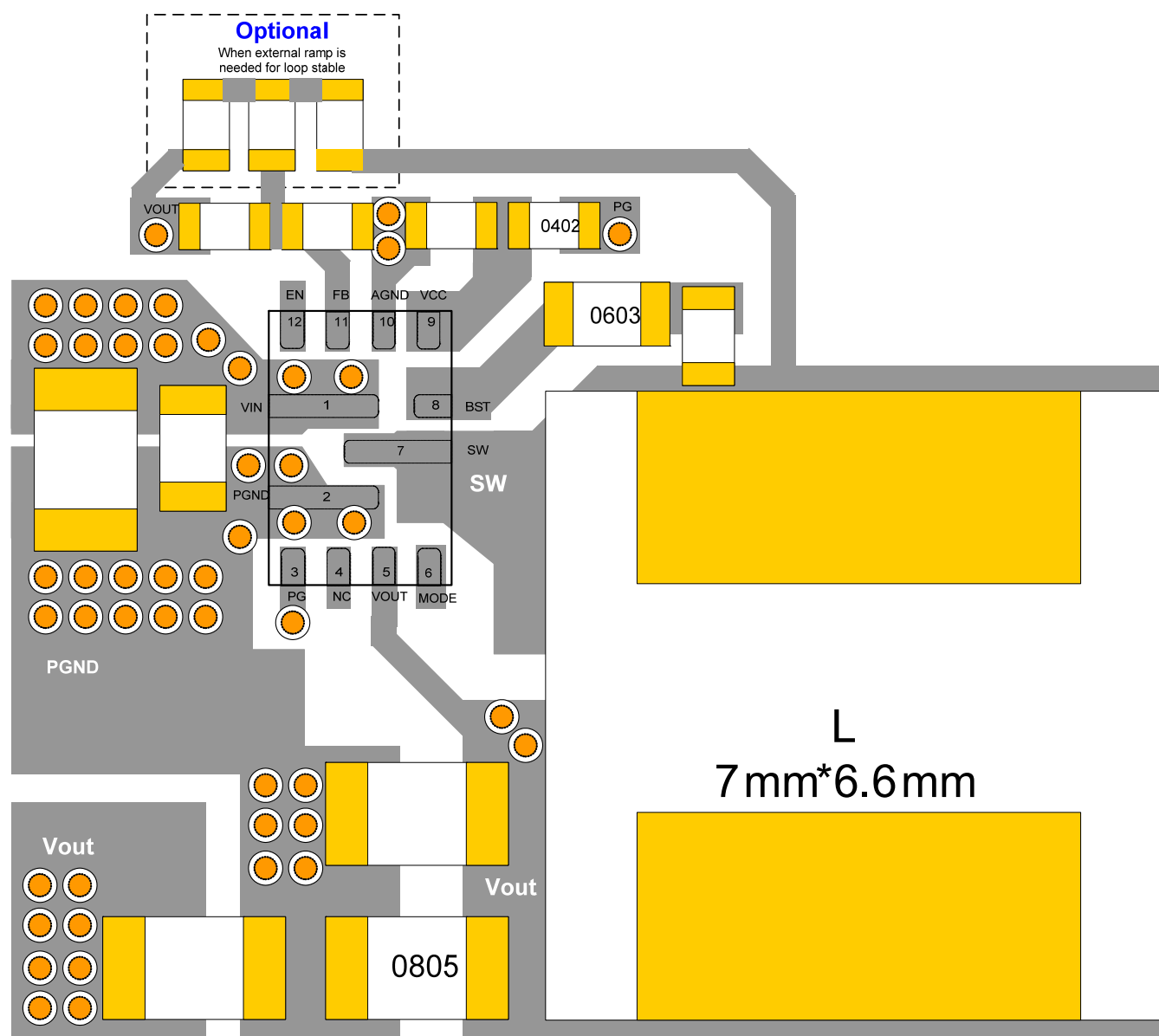
Figure 10: Recommend Layout
