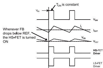
Figure 2: Heavy-Load Operation
