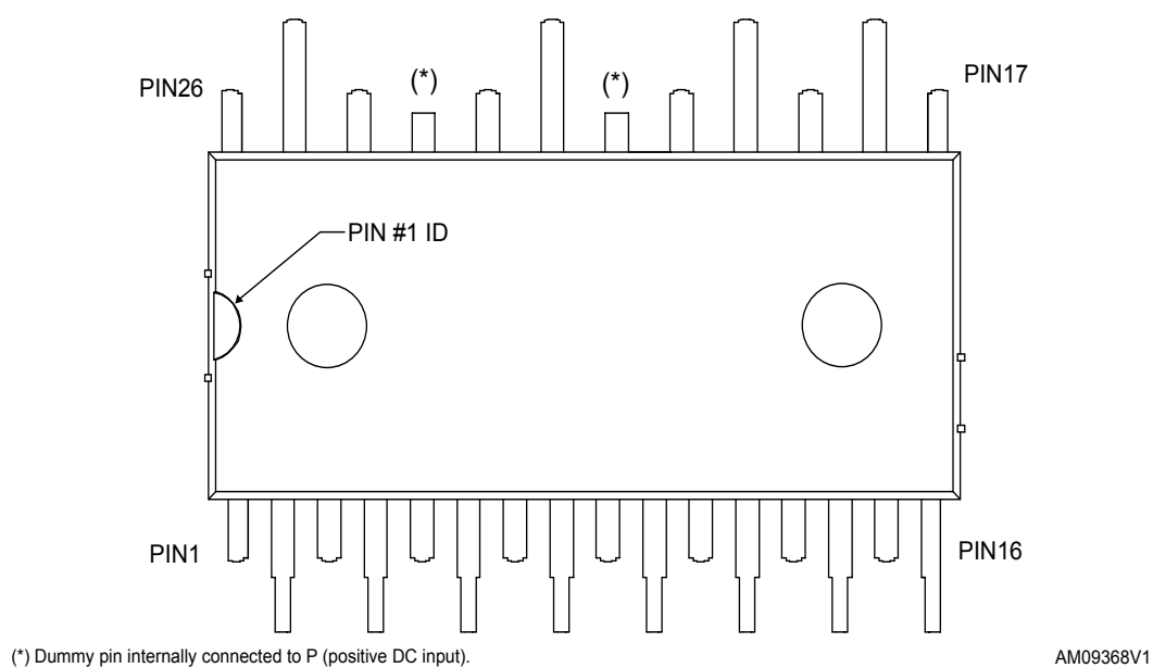
Figure 2. Pin layout (top view)
