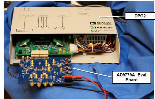
8 Evaluation Board
