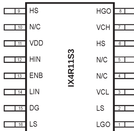
16-PIN SOIC
