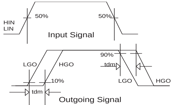
Figure 6. Definitions of Delay Matching Waveforms
