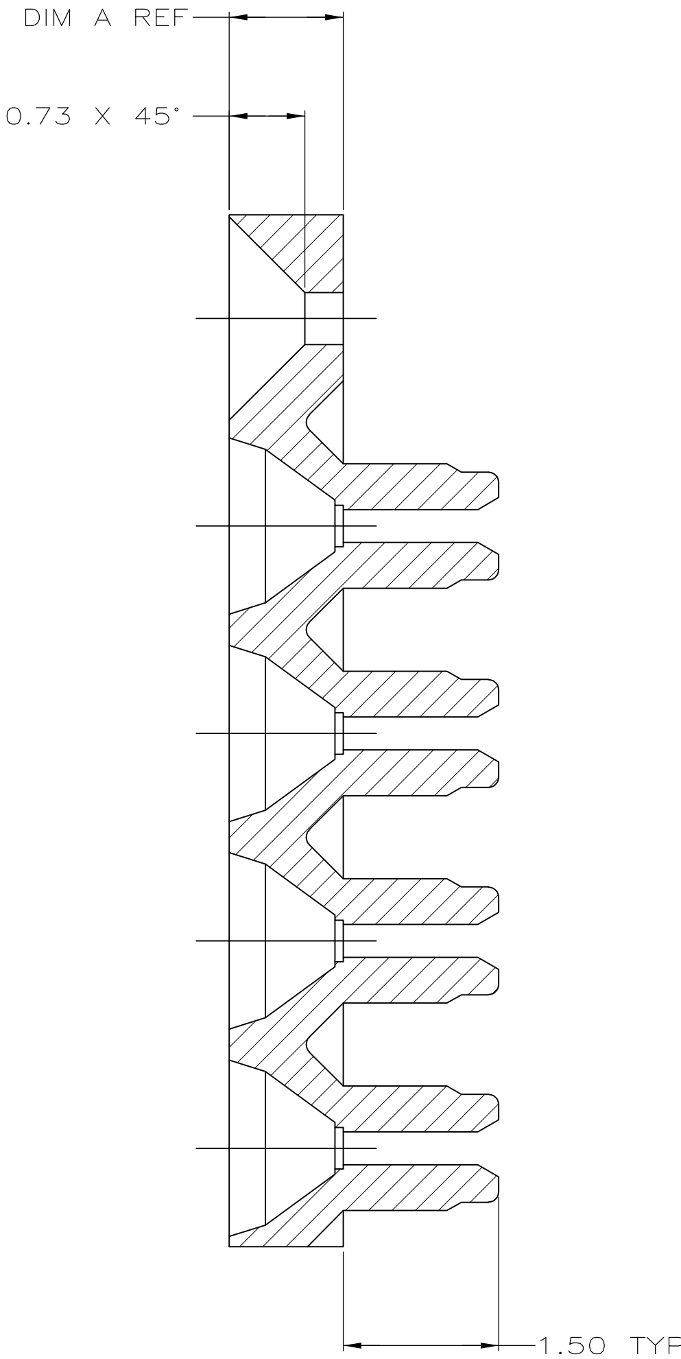
SECTION B-B SCALE 20:1
