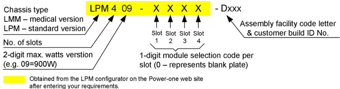
Fig.3 LPM 4-Slot model part number description
