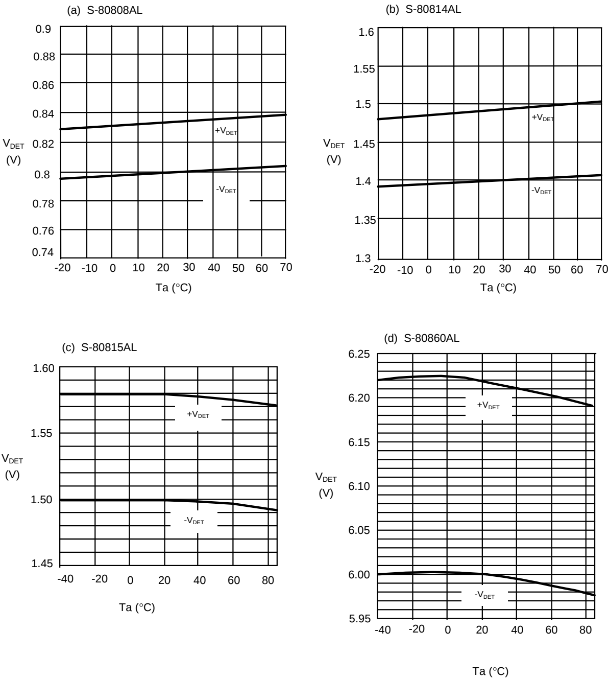
(1) Detection voltage ( V_{DET} ) - Temperature ( T_a )
