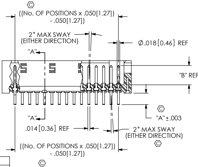
FIG 1 (TFM-115-01-X-S-XX SHOWN)
