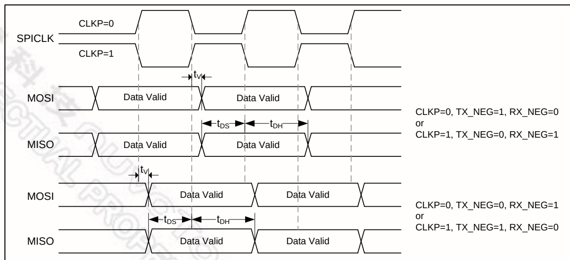
Figure 7.6-1 SPI Master Mode Timing
