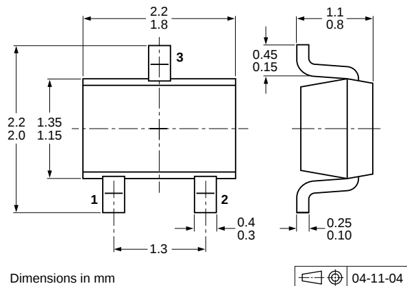
Fig 15. Package outline PDTC143EU (SOT323/SC-70)
