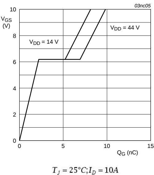
Fig 7. Gate-source voltage as a function of gate charge; typical values
