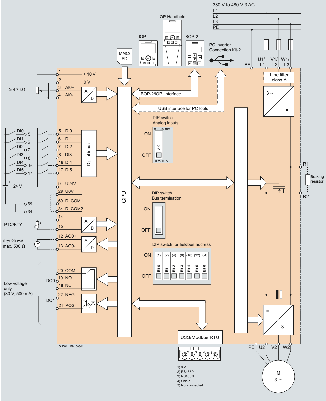
Connection example SINAMICS G120C, USS/Modbus RTU version
