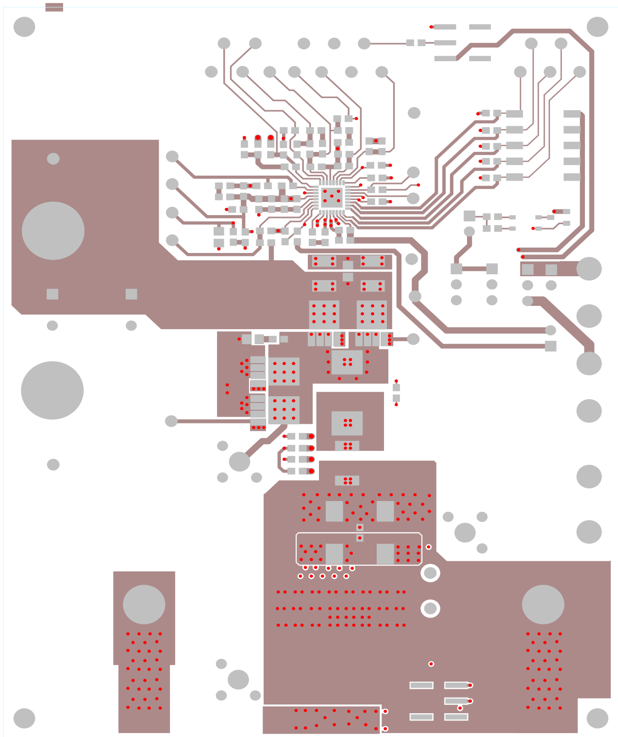
FIGURE 4. ISL6263CEVAL1/1Z and ISL6263DEVAL1Z EVALUATION BOARDS PCB TOP ETCH
