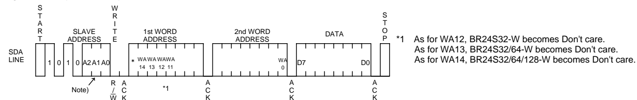
Figure 33. Byte write cycle (BR24S32/64/128/256-W)
