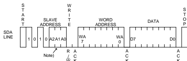
Figure 32. Byte write cycle (BR24S08/16-W)
