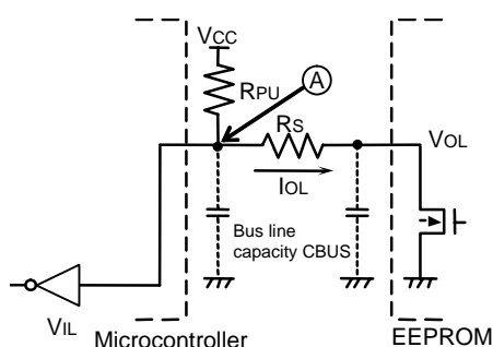
Figure 51. I/O circuit
