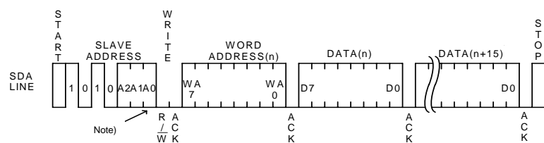
Figure 34. Page write cycle (BR24S08/16-W)
