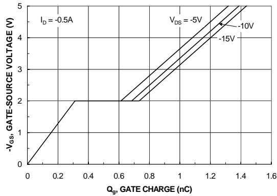
Figure 7. Gate-Charge Characteristics.
