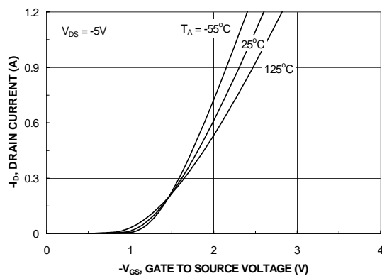
Figure 5. Transfer Characteristics.
