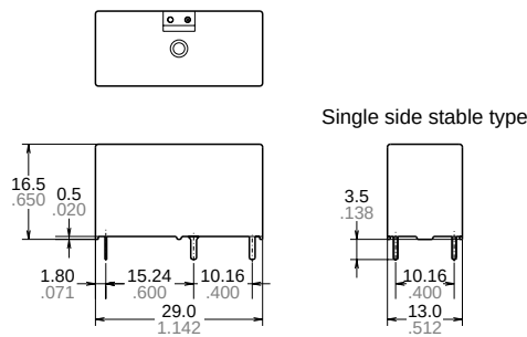
External dimensions
