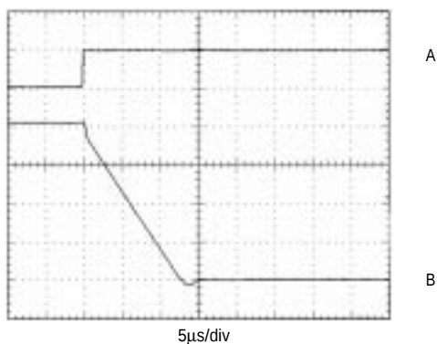
NEGATIVE SETTLING TIME (MAX504)
