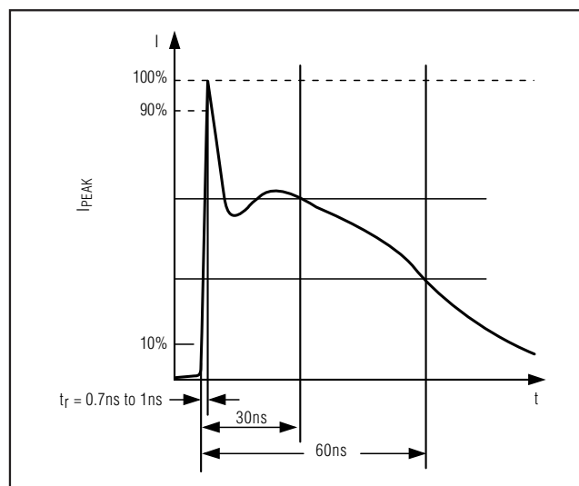
Figure 9b. IEC61000-4-2 ESD Generator Current Waveform
