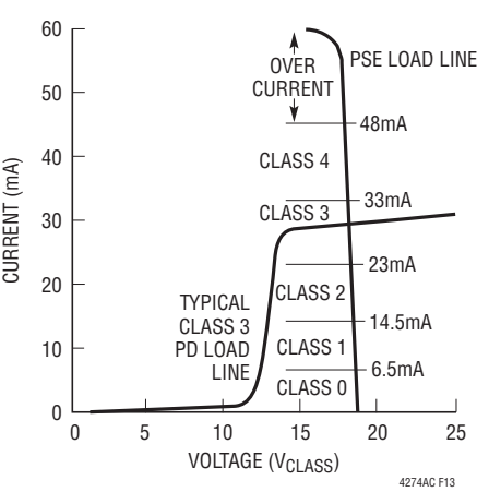
Figure 13. PD Classification
