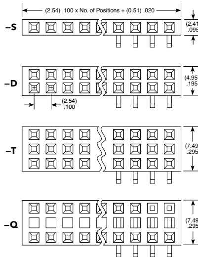
Through-hole
