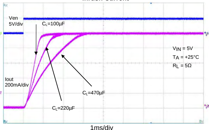
Inrush Current
