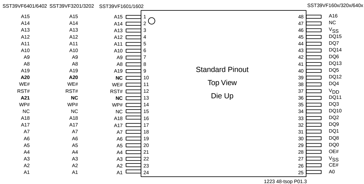
FIGURE 1: PIN ASSIGNMENTS FOR 48-LEAD TSOP
