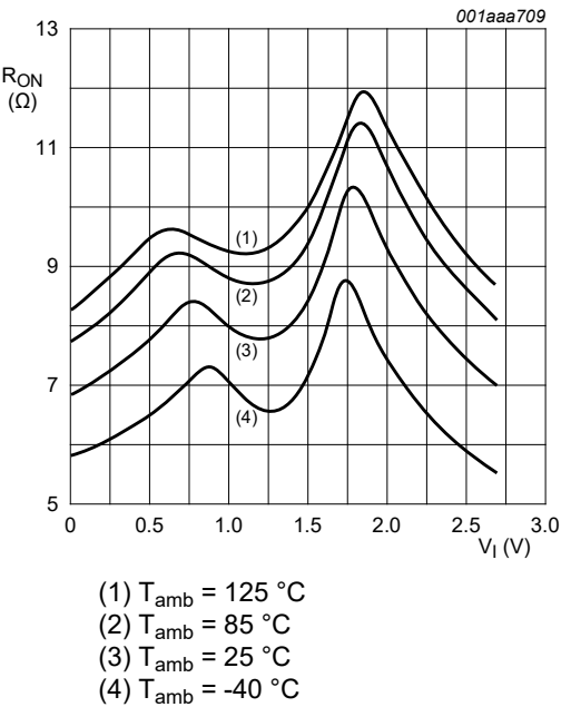
Fig. 9. ON resistance as a function of input voltage; V_{\text{CC}} = 2.7\text{ V}
