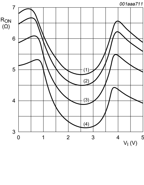
Fig. 11. ON resistance as a function of input voltage; V_{\text{CC}} = 5.0\text{ V}
