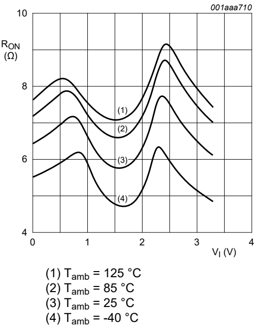
Fig. 10. ON resistance as a function of input voltage; V_{\text{CC}} = 3.3\text{ V}
