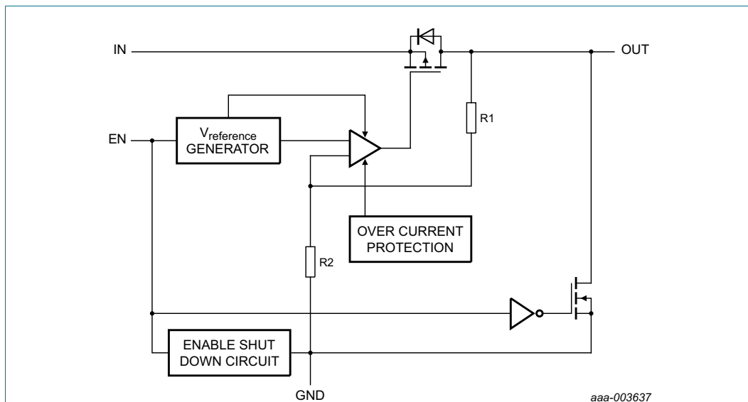
Fig 2. Block diagram of LD6805K/xxP (auto discharge function)
