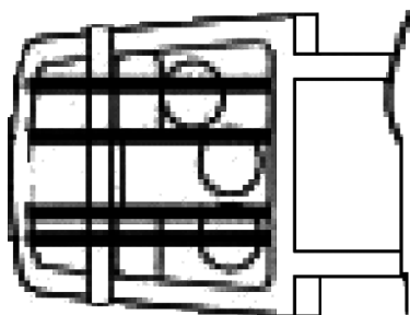
Detail of blades in stripping jaw showing three-level strip.
