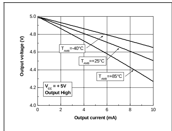
Output sourcing current vs Output voltage @ V_{CC} = +5V
