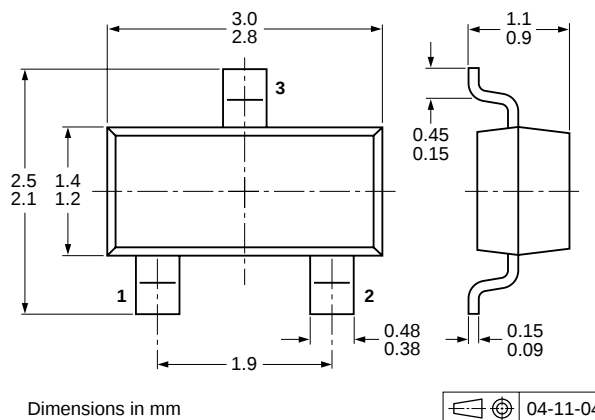
Fig 7. Package outline MMBD4148 (SOT23/TO-236AB)
