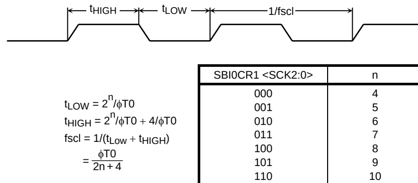
Figure 3.12.6 Clock Source
