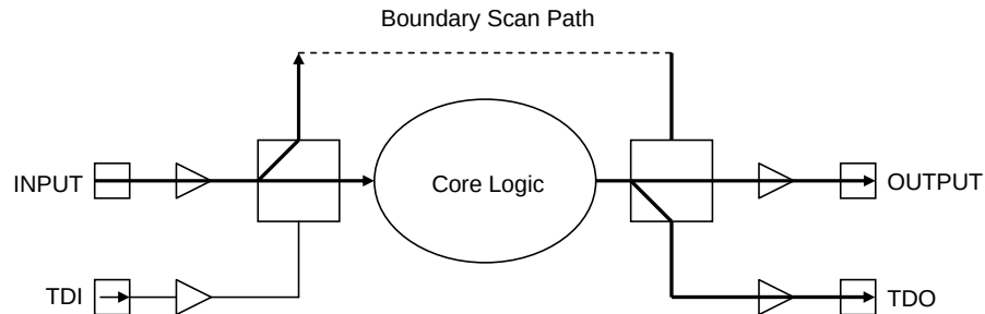
Figure 6.4.2 Test Data Flow While SAMPLE is Selected
