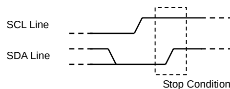
Figure 3.12.9 Generating a Stop Condition
