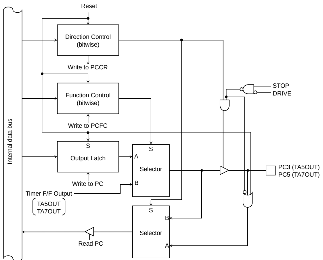
Figure 3.5.29 Port C (PC3, PC5)
