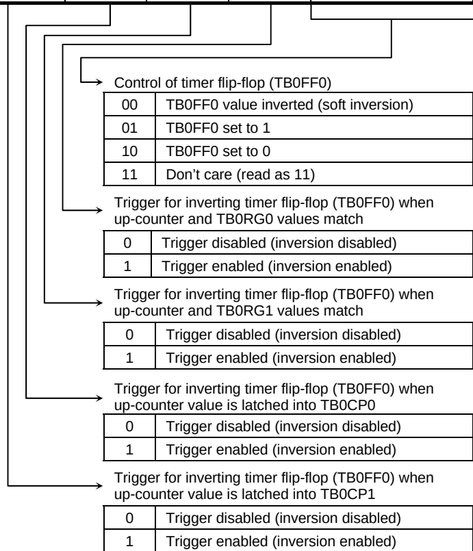
Figure 3.10.16 TMRB Registers
