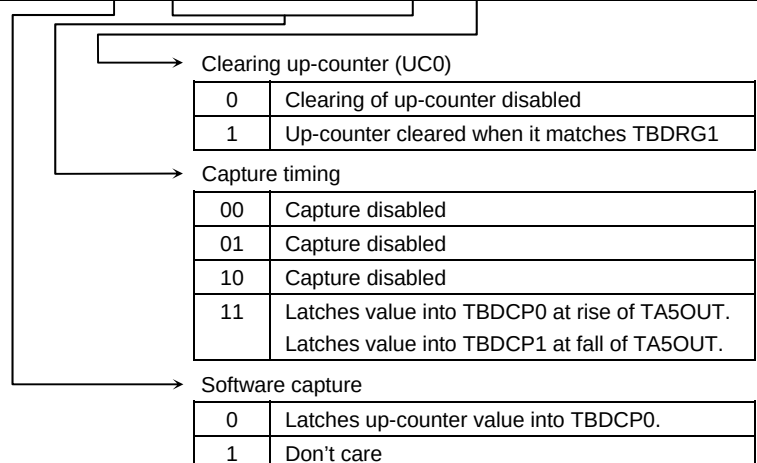
Figure 3.10.15 TMRB Registers
