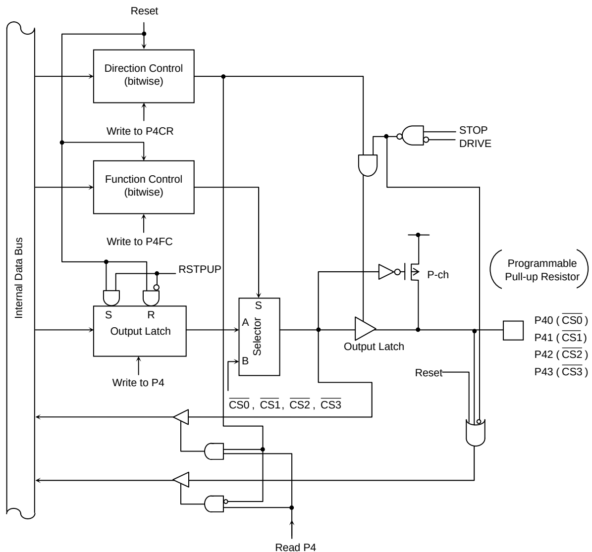
Figure 0.12 Port 4 (P40-P43)
