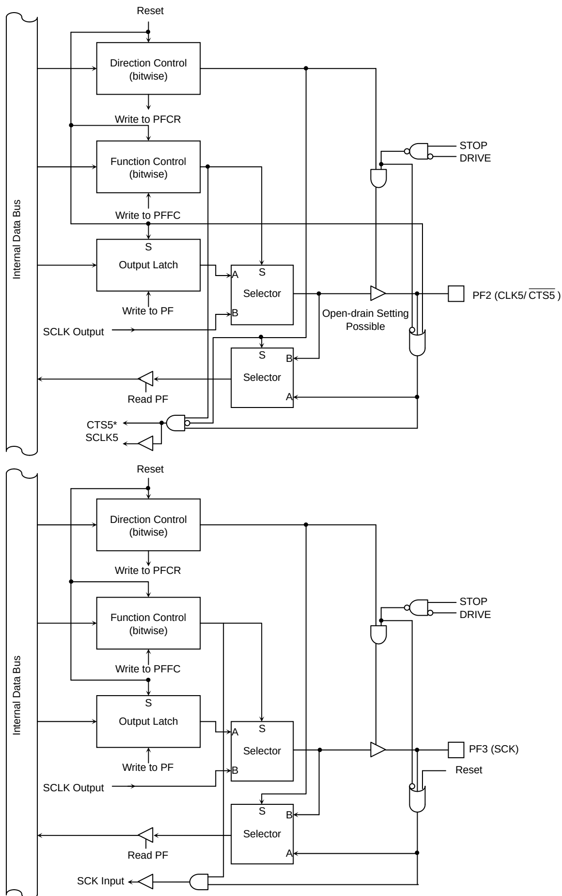
Figure 3.5.44 Port F (PF2, PF3)
