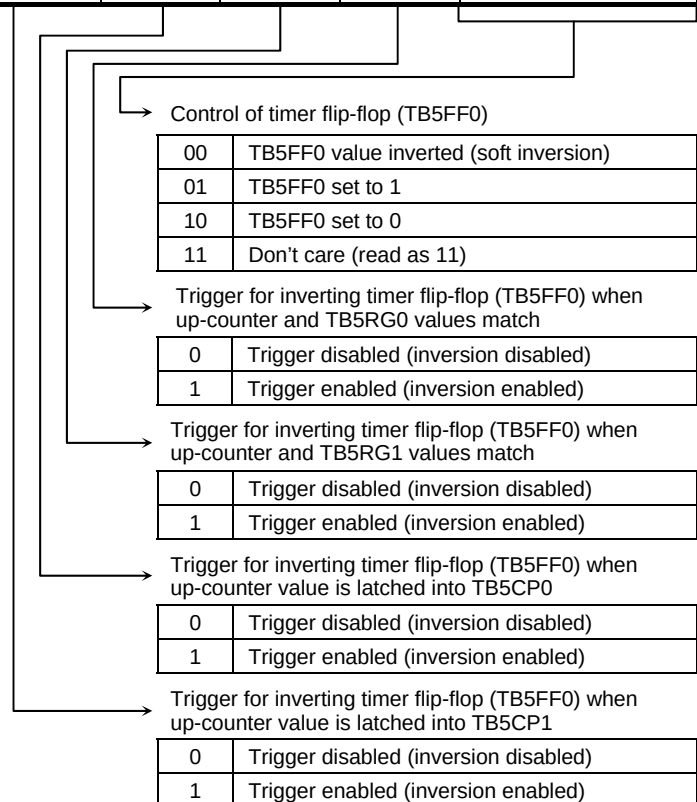
Figure 3.10.21 TMRB Registers
