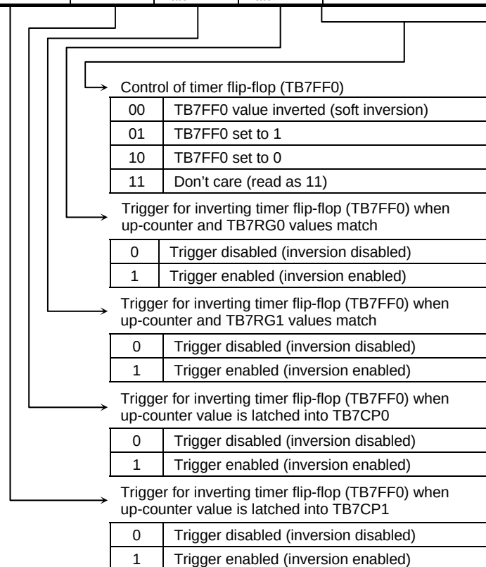
Figure 3.10.23 TMRB Registers
