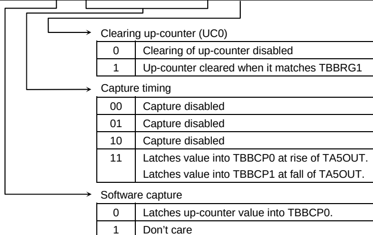
Figure 3.10.14 TMRB Registers
