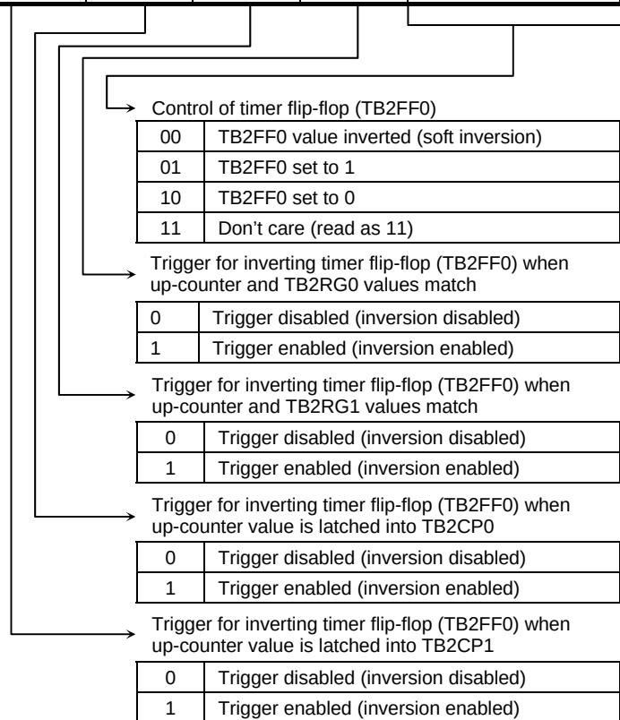
Figure 3.10.18 TMRB Registers
