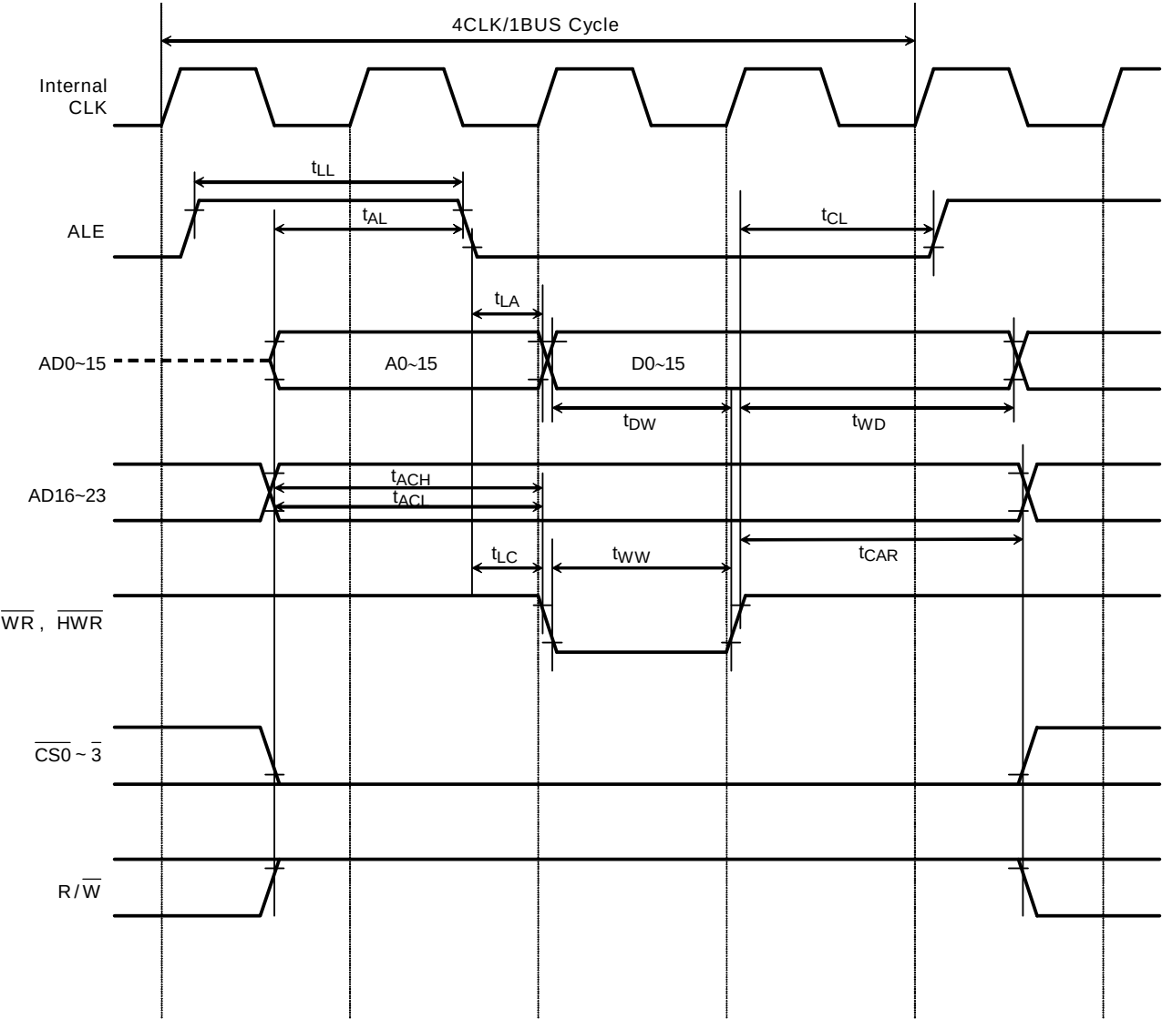
(4) Write Cycle Timing (ALE = 1.5, No-Wait)
