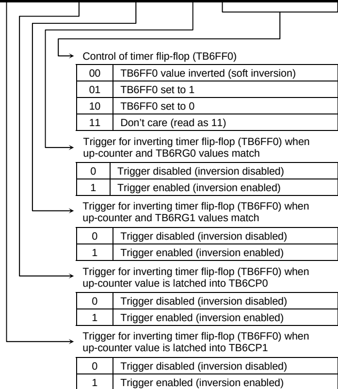
Figure 3.10.22 TMRB Registers
