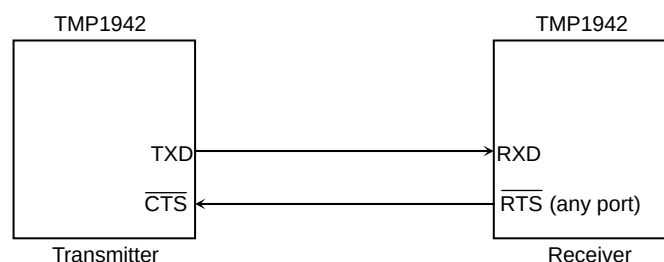
Figure 3.11.4 Handshaking Function
