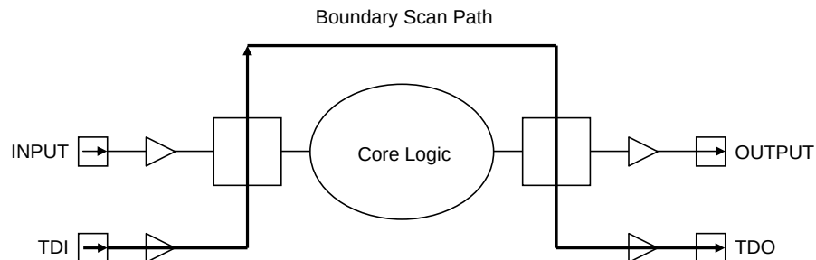
Figure 6.4.3 Test Data Flow While PRELOAD is Selected
