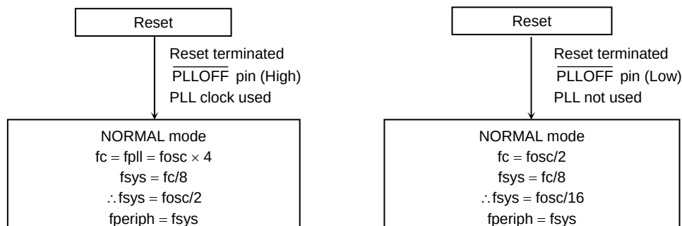
Figure 3.3.1 State Transition Diagrams for Different Modes
