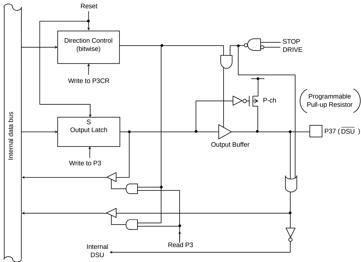
Figure 0.10 Port 3 (P37)
