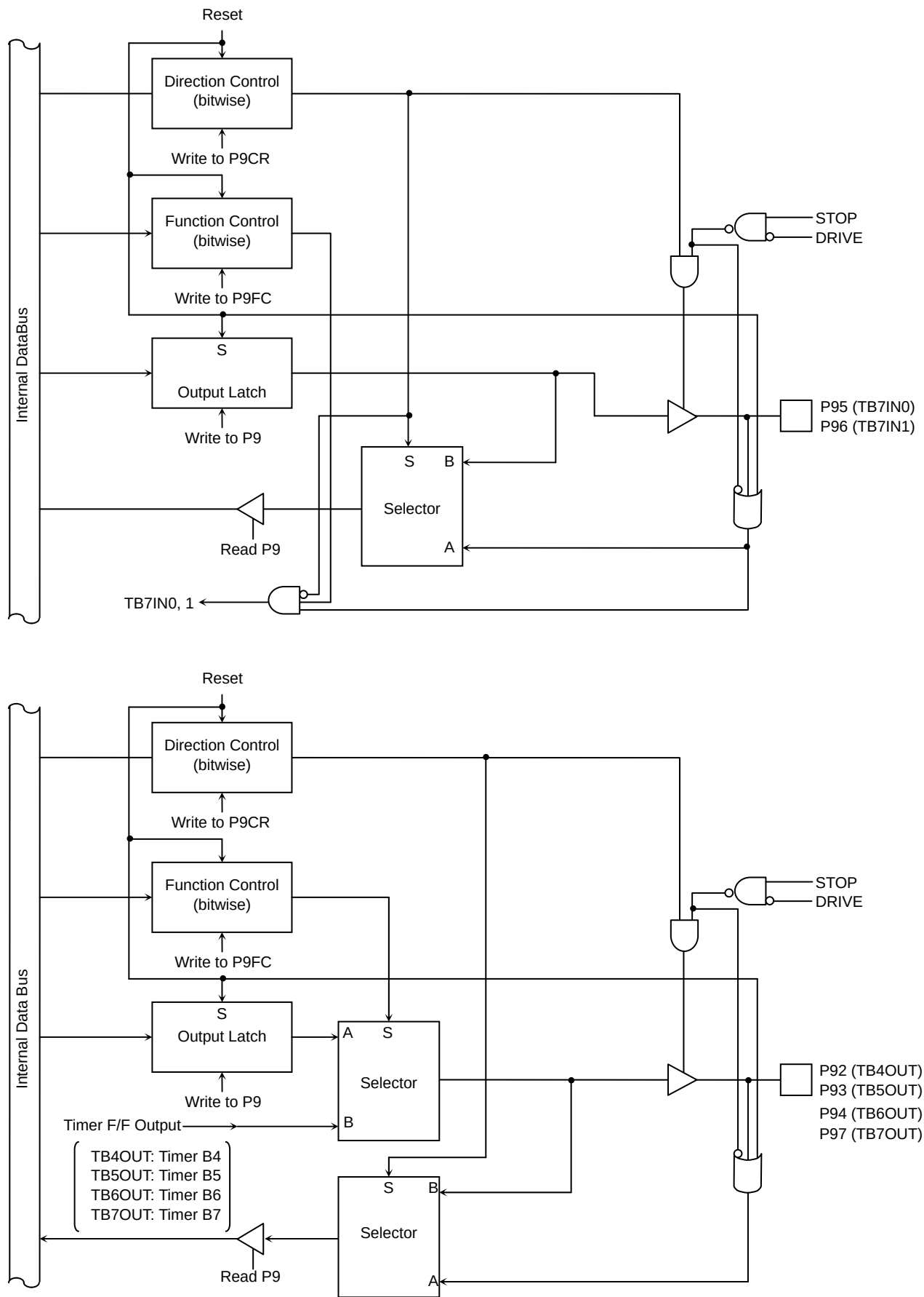
Figure 0.20 Port 9 (P92-P97)
