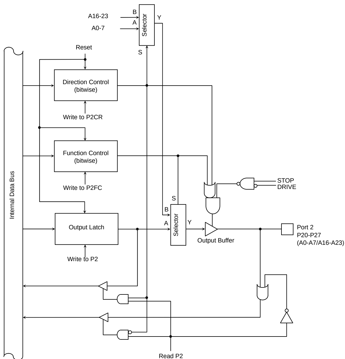
Figure 0.5 Port 2 (P20-P27)
