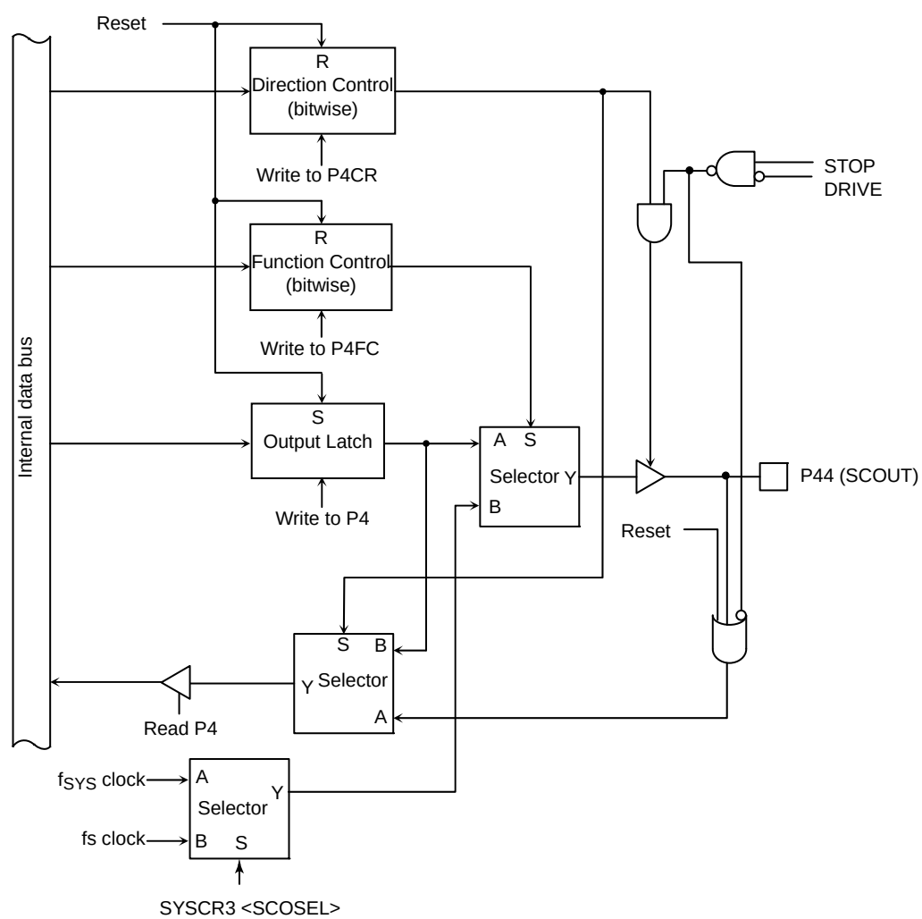
Figure 0.13 Port 4 (P44)
