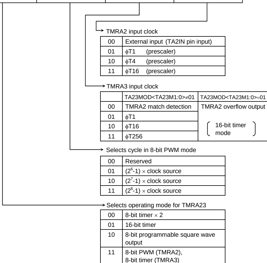
Figure 3.9.7 TMRA Registers
