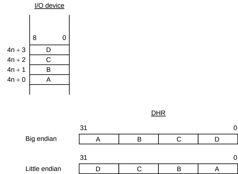
Figure 3.8.14 Data Packing and Unpacking
