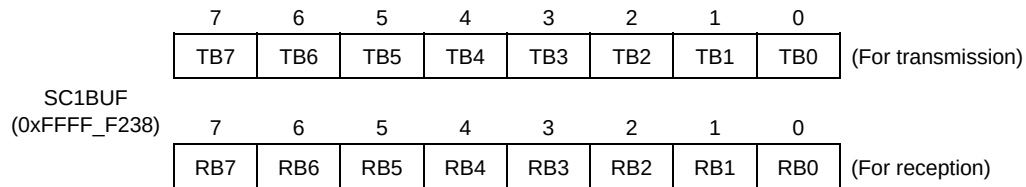
Figure 3.11.32 Serial Transmit/Receive Buffer Register (SC1BUF, for SIO1)
