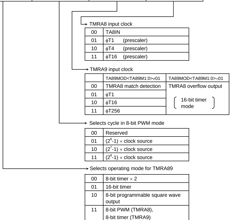
Figure 3.9.10 TMRA Registers
