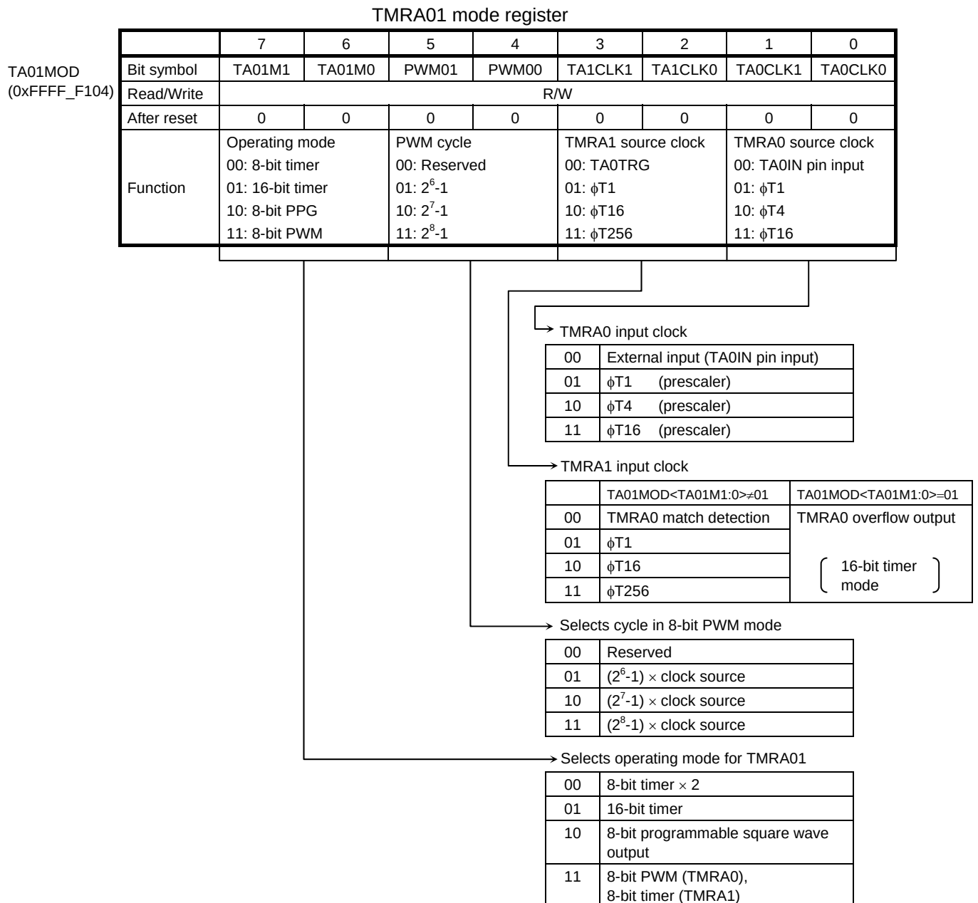
Figure 3.9.6 TMRA Registers
