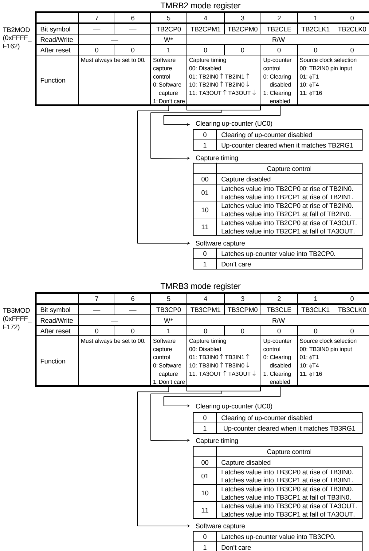
Figure 3.10.10 TMRB Registers
