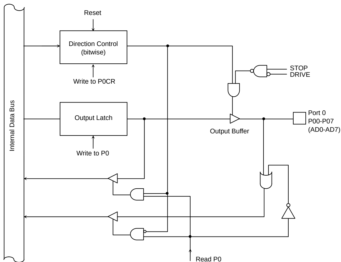
Figure 0.1 Port 0 (P00-P07)
