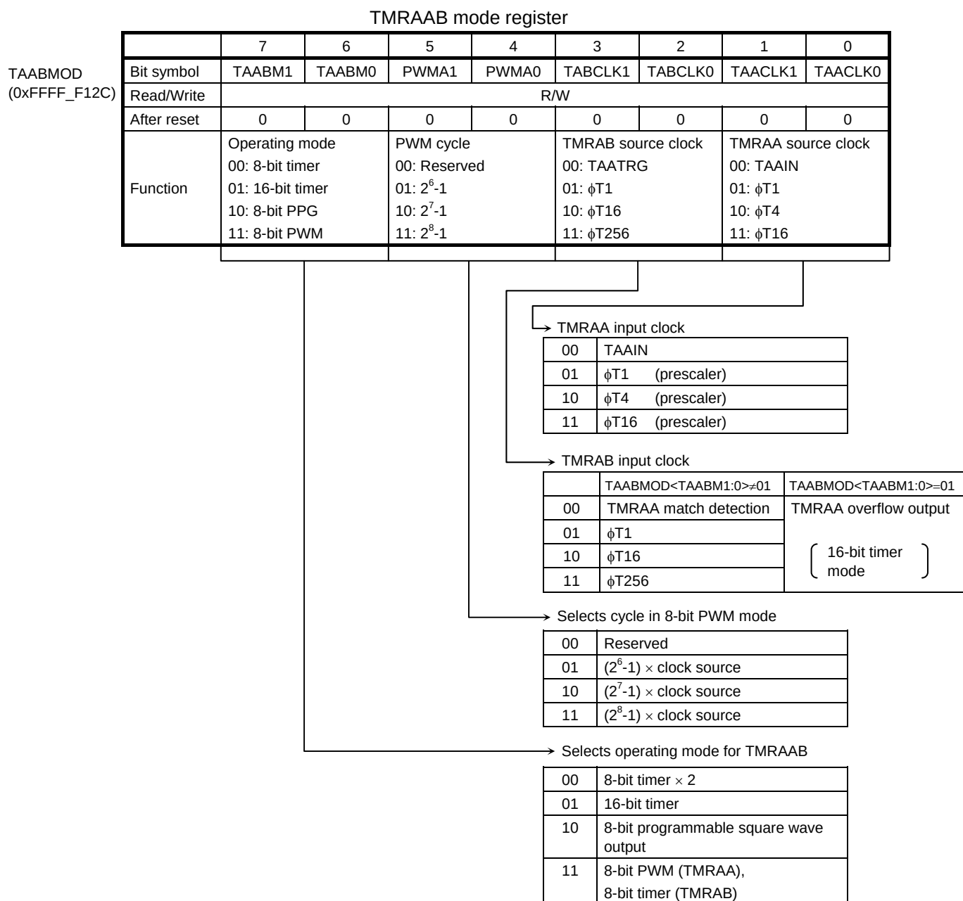
Figure 3.9.11 TMRA Registers
