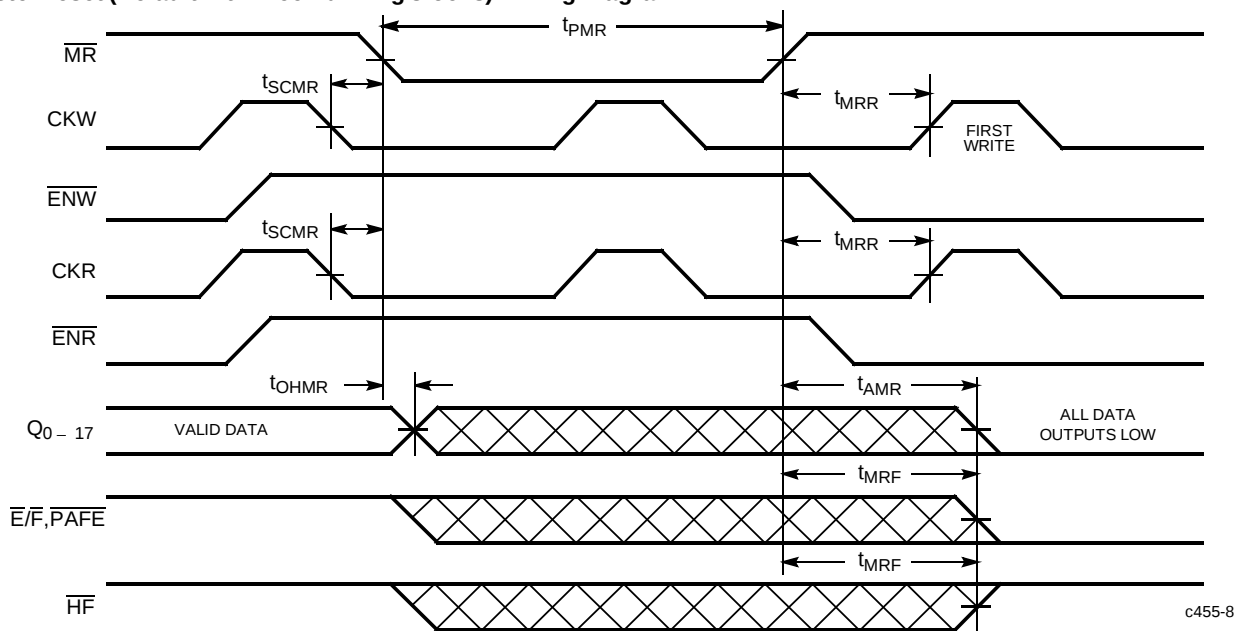
MasterReset (Default with Free-Running Clocks) Timing Diagram [17, 18, 19, 20]
