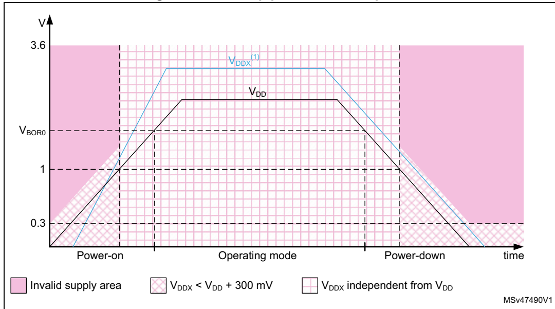
Figure 4. Power-up/power-down sequence
