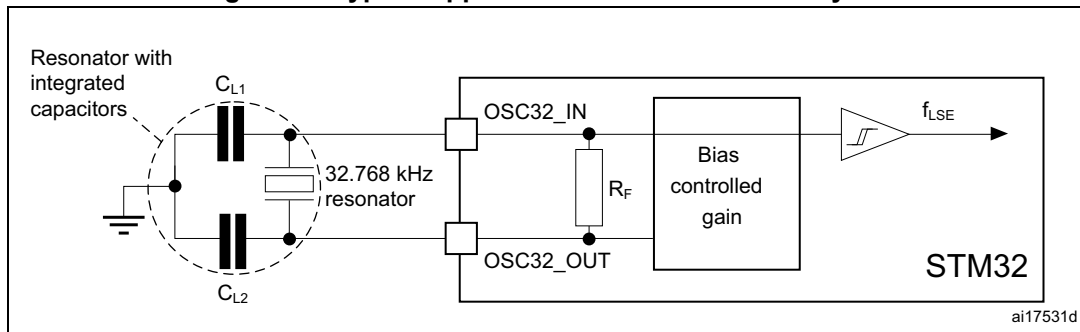
Figure 24. Typical application with a 32.768 kHz crystal
