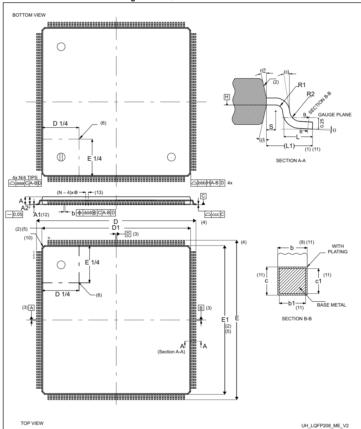
Figure 77. LQFP208 - Outline (15)
