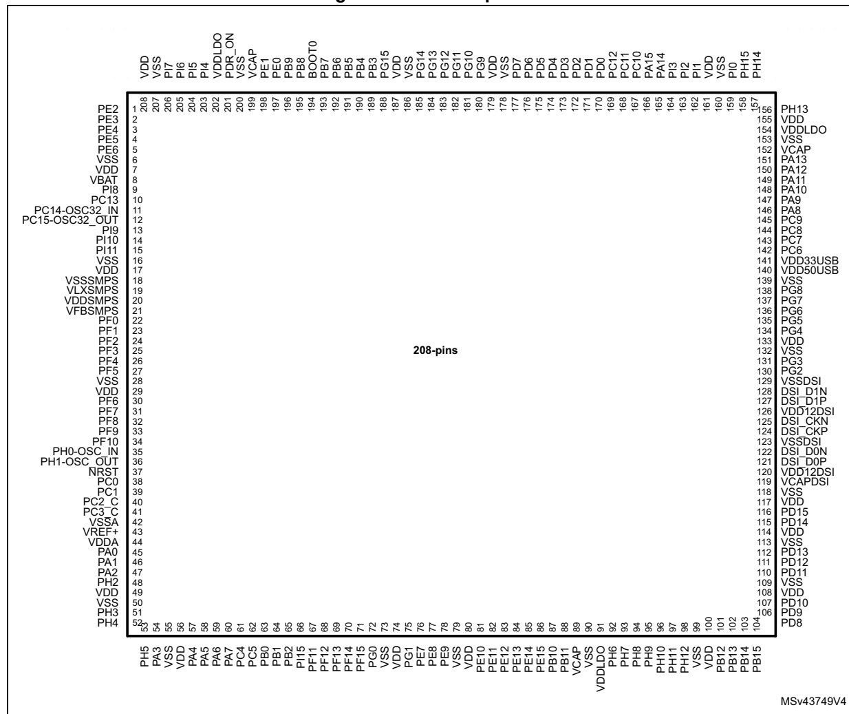
Figure 9. LQFP208 pinout
