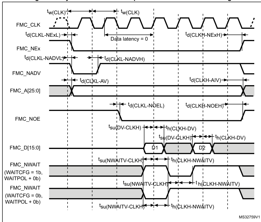
Figure 34. Synchronous non-multiplexed NOR/PSRAM read timings
