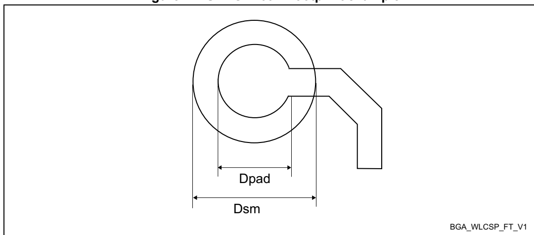
Figure 74. UFBGA169 - Footprint example
