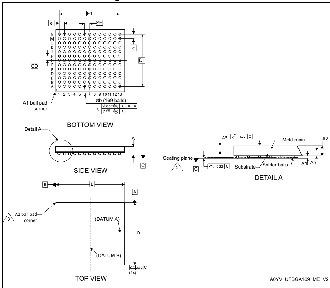
Figure 73. UFBGA169 - Outline
