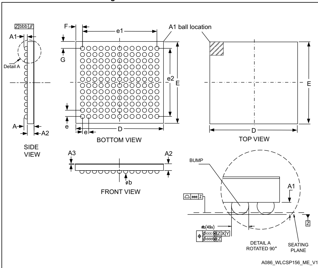
Figure 70. WLCSP156 - Outline
