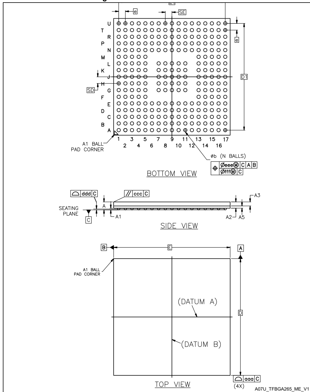
Figure 79. TFBGA240+25 - Outline
