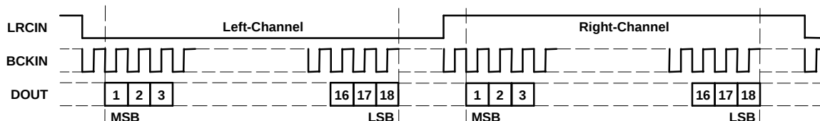
Figure 20. Audio Data Input/Output Format (Formats 4 and 5)
