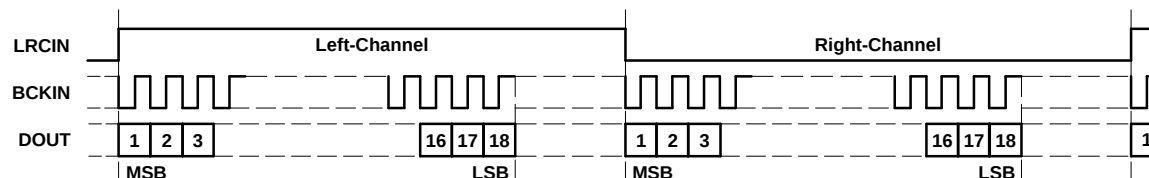
Figure 18. Audio Data Input/Output Format (Formats 0 and 1)
