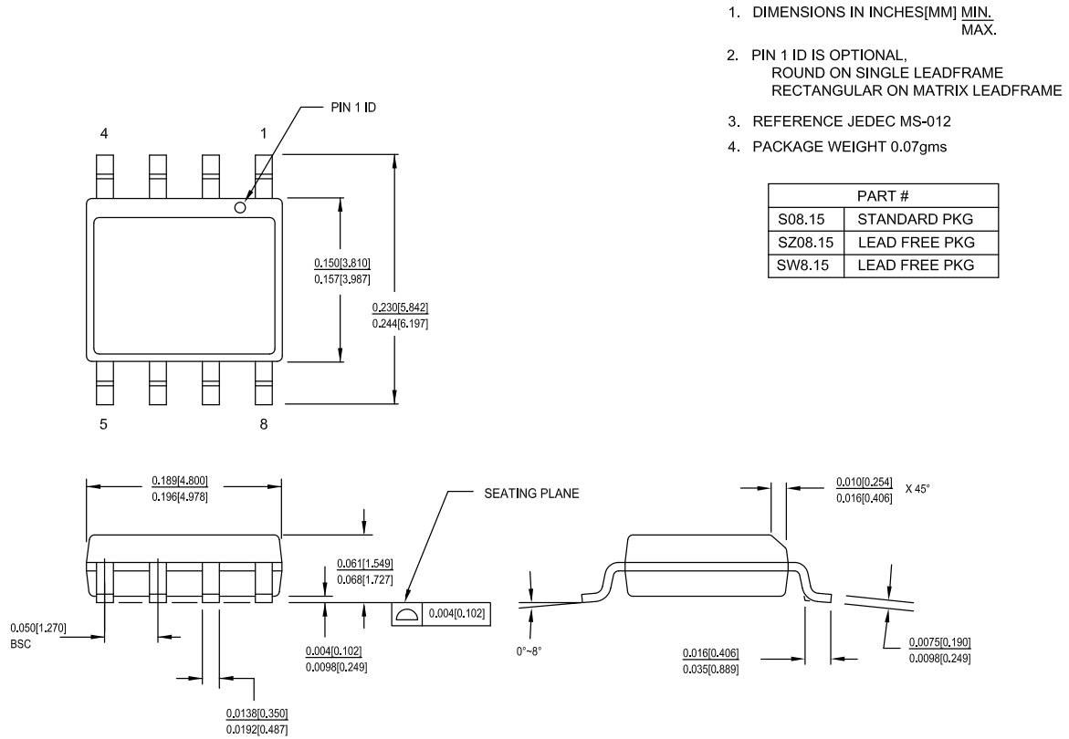
Figure 17. 8-pin SOIC (150 Mils) S08.15/SZ08.15 Package Outline, 51-85066
