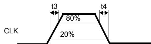
Figure 7. Rise and Fall Time Definitions
