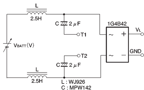
Fig. 10 Trunk circuit
