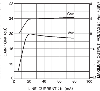
Fig. 3 MF Line current
