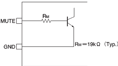
Fig. 15 Mute input equivalent circuit
