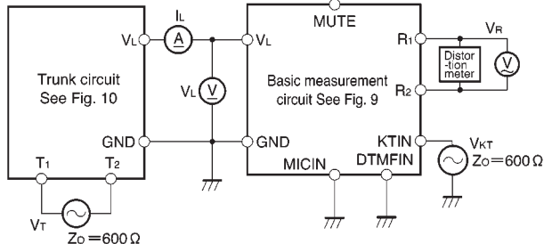
Fig. 12 Reception system measurement circuit
