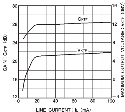
Fig. 7 Piezoelectric KT Line current
