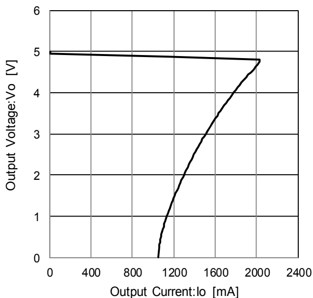
Figure 39. Load Regulation
