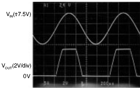
FIGURE 2. A \pm 7.5V Input Signal Greatly Exceeds the 5V Supply in Figure 3 Causing No Phase Inversion Due to R_I
