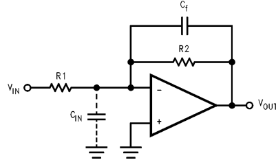
FIGURE 4. Cancelling the Effect of Input Capacitance
