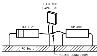
FIGURE 8. Air Wiring (Input pins are lifted out of PC board and soldered directly to components. All other pins connected to PC board).
