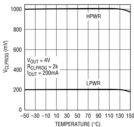
V_{CLPROG} vs Temperature at I_N = 500mA
