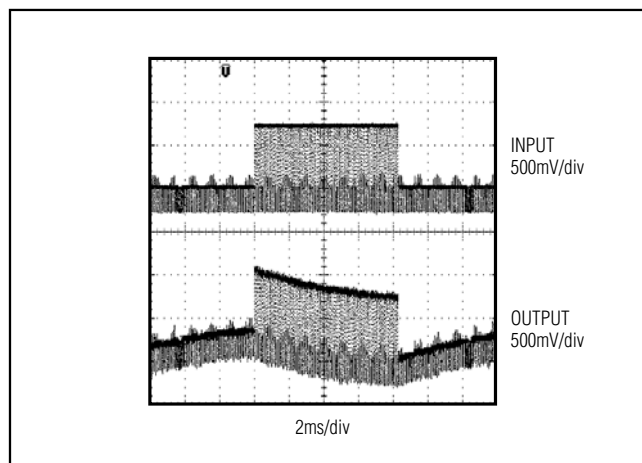
Figure 1. AC-Coupled Output
