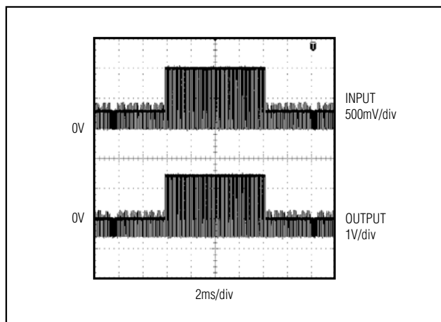
Figure 2. DirectDrive Output
